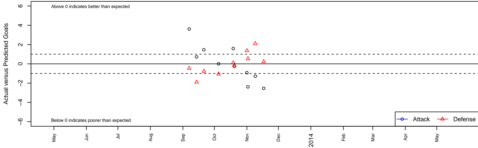
Davis Legacy Stampede G01 Dots are actual minus expected GF (blue circles) and GA (red triangles). Blue line is smoothed change in attack strength. Red is smoothed change in defense strength.
